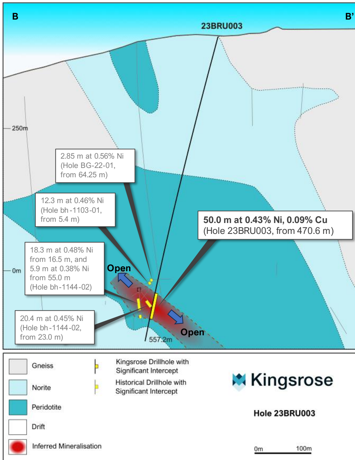
Figure 6: Cross section (Section B-B') showing hole 23BRU003.
