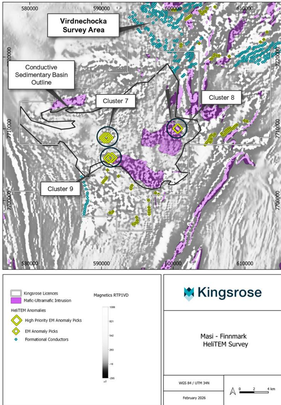
Figure 3: HelITEM anomaly picks overlain on RTP1VD magnetic, Masi area.
