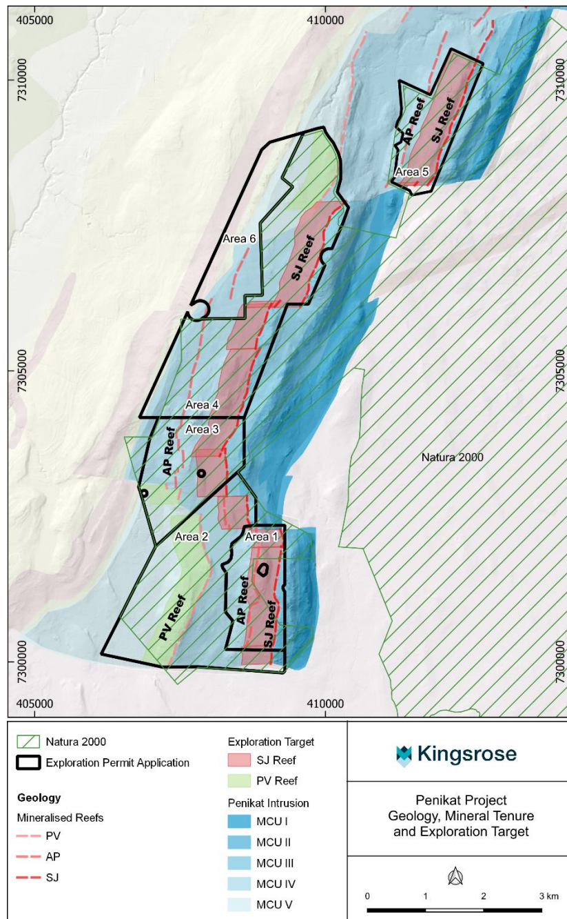
Figure 4: Kingsrose Mineral Tenure and Geology of the Penikat Project, Finland.
