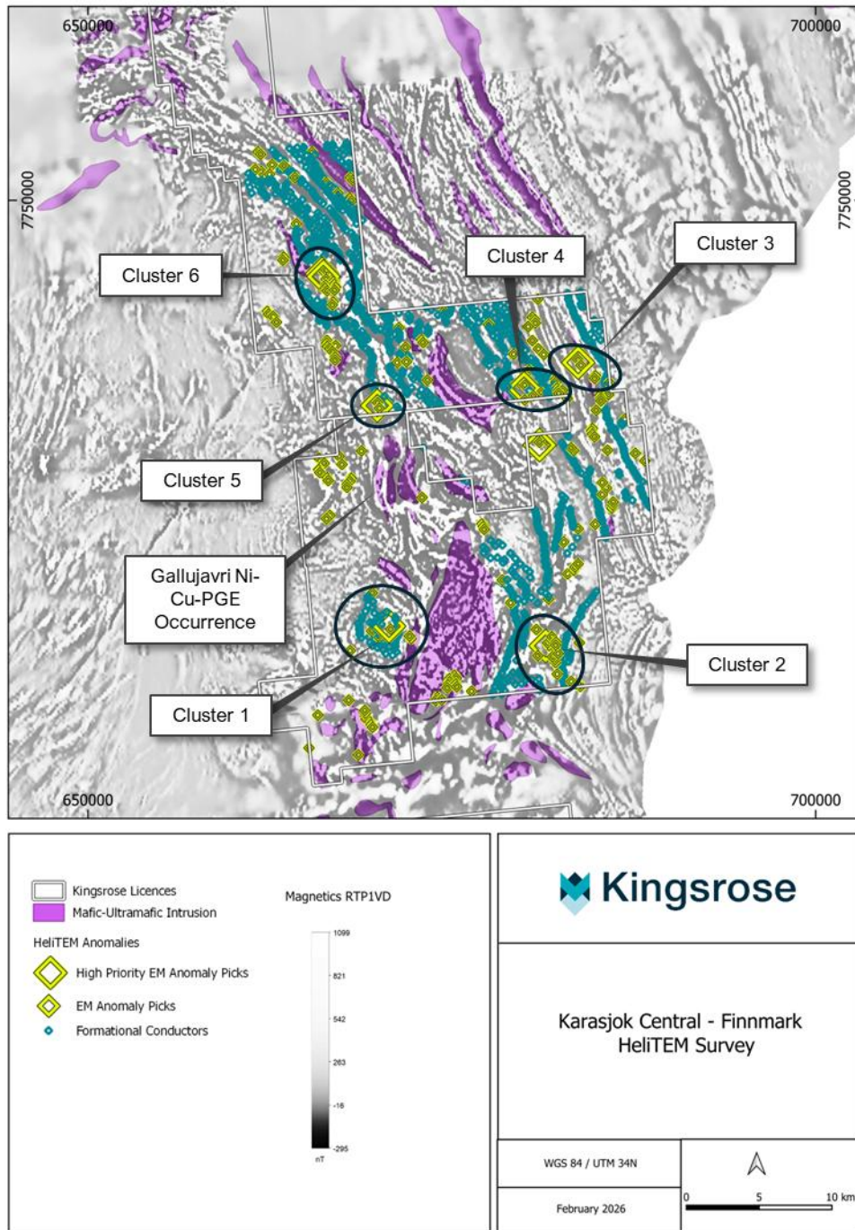
Figure 2: HelITEM anomaly picks overlain on RTP1VD magnetic, Karasjok Central area.
