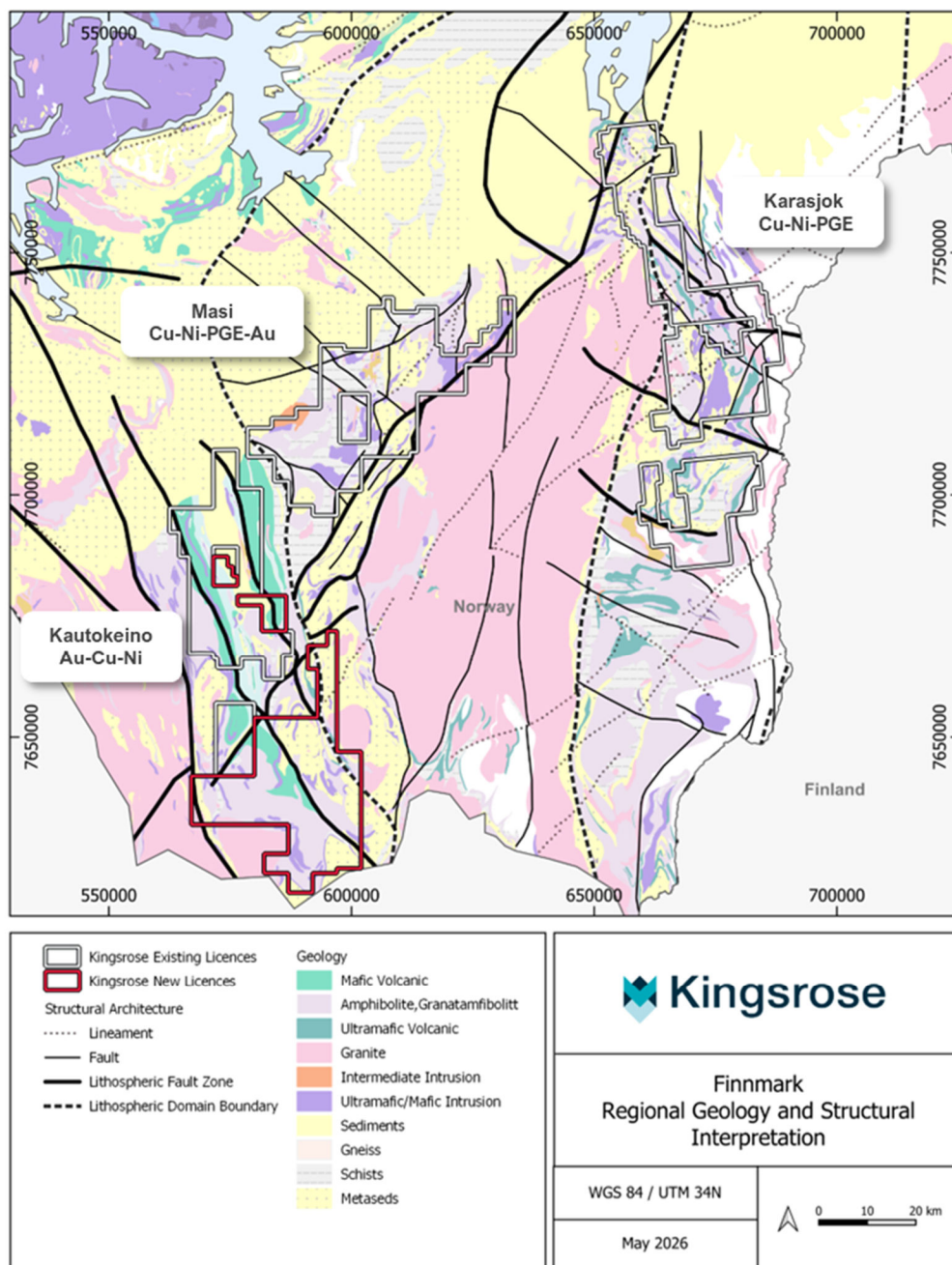
Figure 2: New licences over regional geology and Kingsrose architecture interpretation, Finnmark Project.
