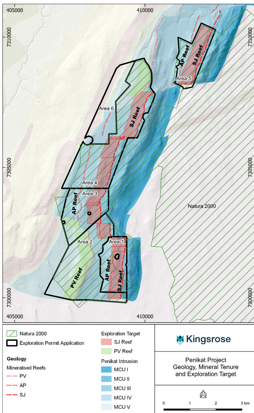
Figure 3: Kingsrose Mineral Tenure and Geology of the Penikat Project, Finland.
